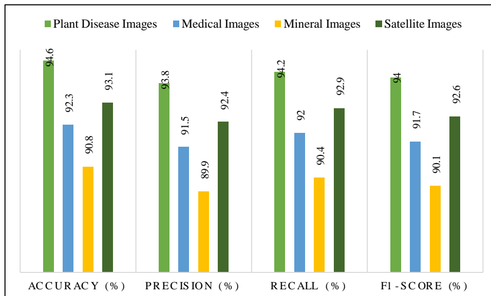
Figure 2. Classification performance metrics (Accuracy, Precision, Recall, F1-score) of the proposed deep learning model
